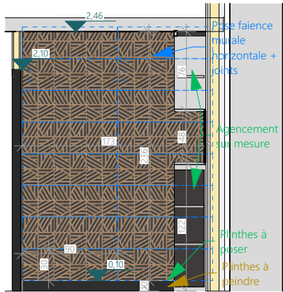
Coupe LL
